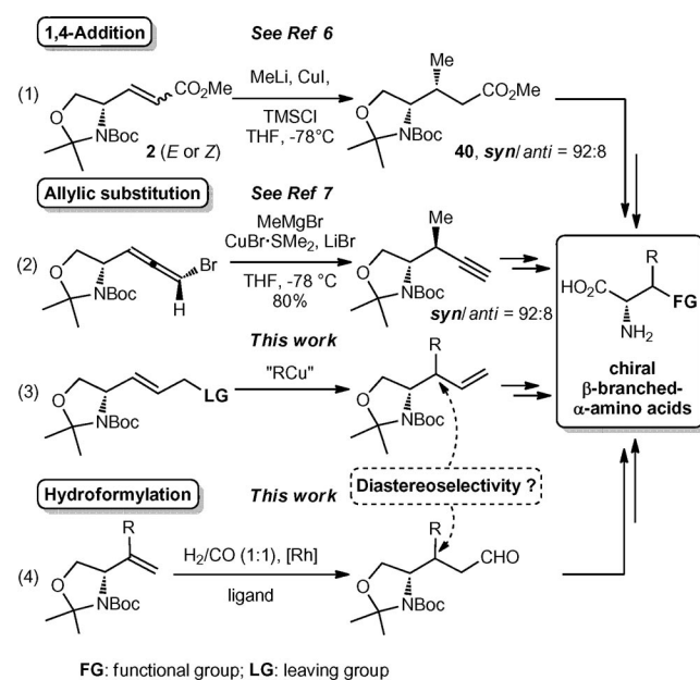
Figure 1. Diastereoselective approaches to \beta -branched \alpha -amino acids.
