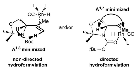
Figure 4. Proposed rationale for the observed syn diastereoselectivity.
