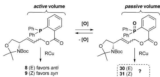
Figure 2. o DPPB on/off switch for S_N2' stereodivergency.
