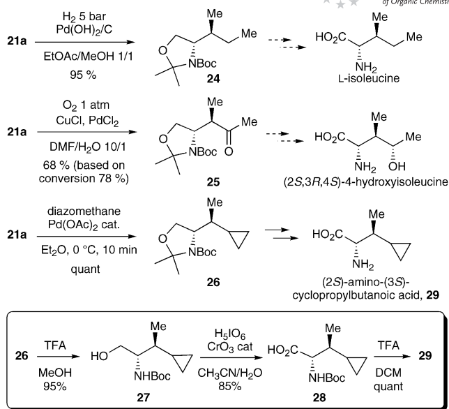
Scheme 2. Functionalization of the terminal olefin for the preparation of \beta -branched \alpha -amino acids.
