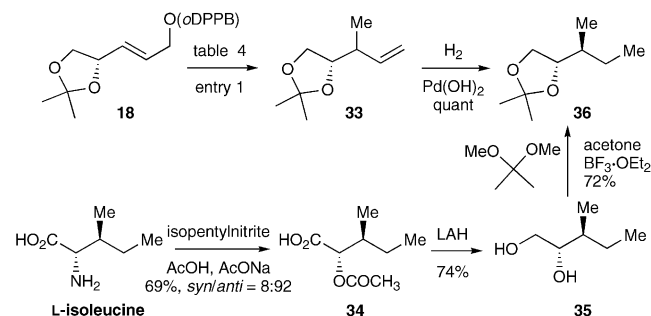
Scheme 3. Correlation of the relative stereochemistry of the dioxolane derivatives.
