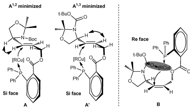
Figure 3. Rationale for the diastereochemical outcome.
